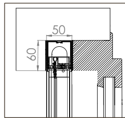
BORA TOP ENCAS STANDARD 20/20
