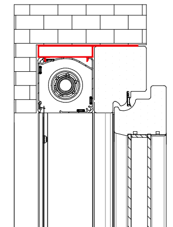
SECTION VERTICALE
