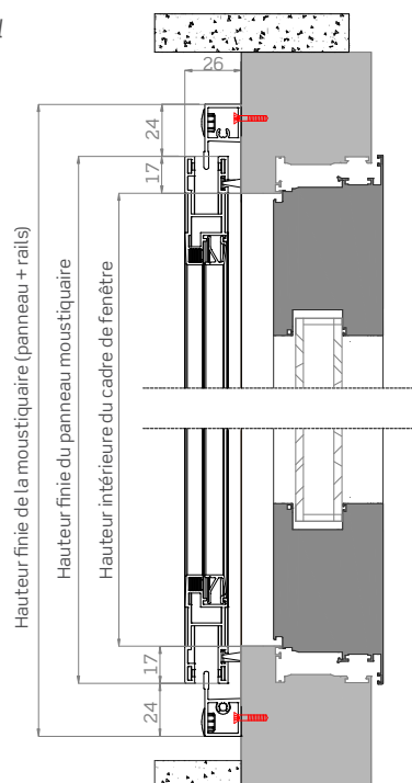
Section verticale
