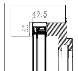
BORA TOP ENCAS DOUBLE MIDI 20/20
