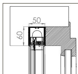
BORA TOP ENCAS STANDARD 50/20
