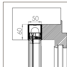
BORA ENCAS STANDARD 20/20
