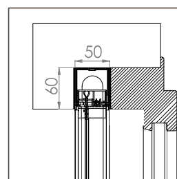
BORA ENCAS STANDARD 50/20
