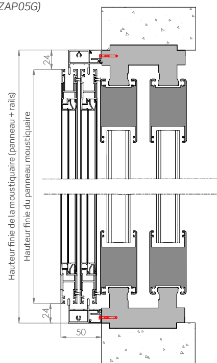
Section verticale
