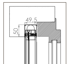
BORA ENCAS DOUBLE MIDI 20/20
