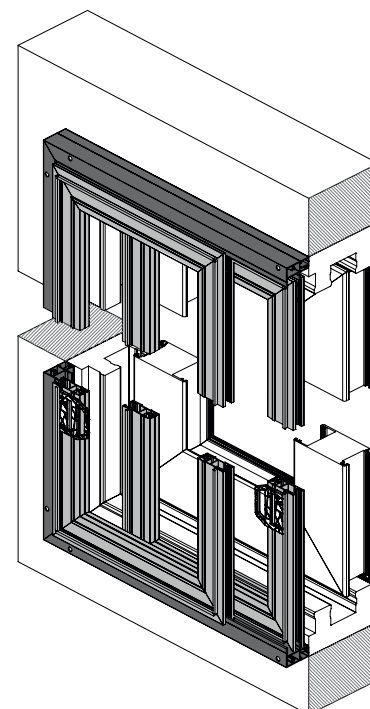
Section verticale
