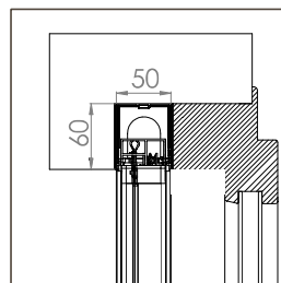
BORA ENCAS DOUBLE STANDARD 20/20
