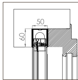
BORA ENCAS STANDARD 50/50
