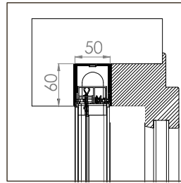
BORA ENCAS STANDARD 50/35
