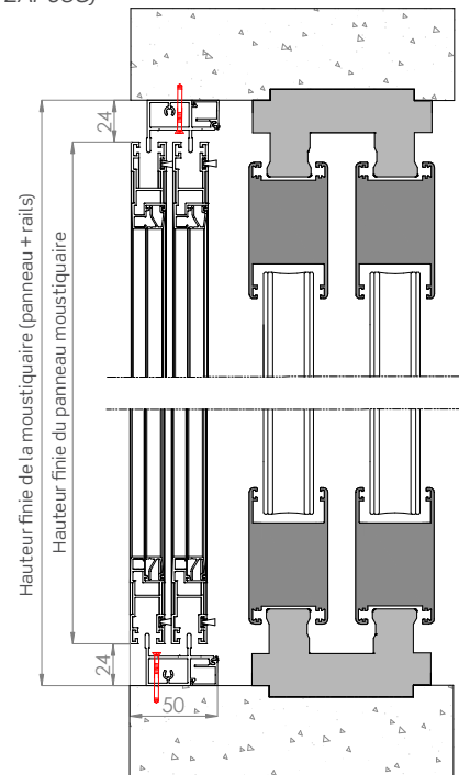
Section verticale
