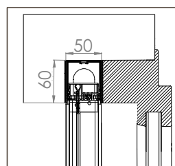
BORA TOP ENCAS STANDARD 50/50
