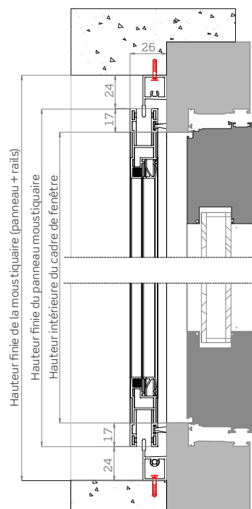
Section verticale
