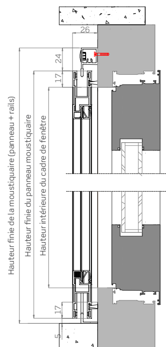
Section verticale
