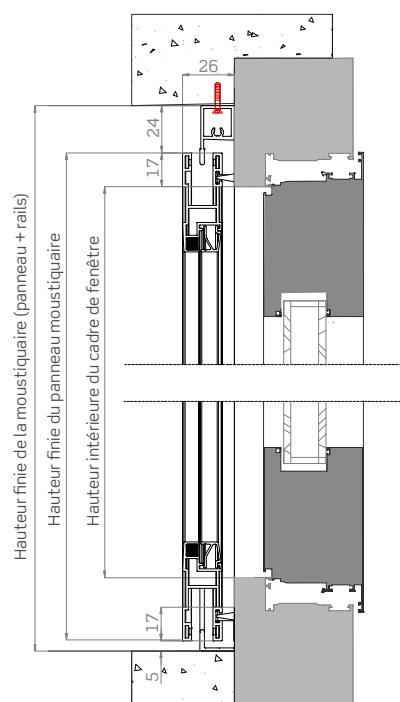
Section verticale
