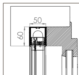
BORA TOP ENCAS STANDARD 50/35
