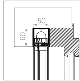
EINBAU-BORA SR STANDARD 20
