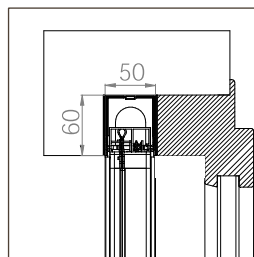
EINBAU-BORA STANDARD 50/20
