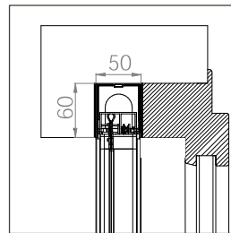
EINBAU-BORA SR STANDARD 35
