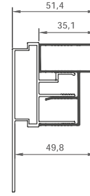
ZCA11Q + ZAG04Q
