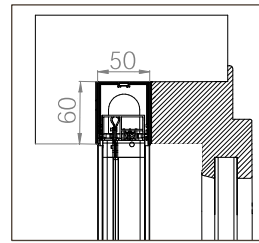
EINBAU-BORA TOP STANDARD 50/50
