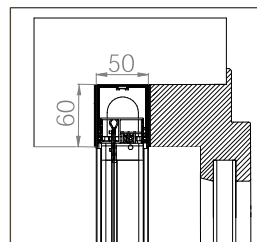
EINBAU-BORA TOP STANDARD 50/20
