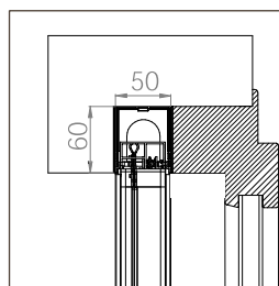
EINBAU-BORA STANDARD 20/20
