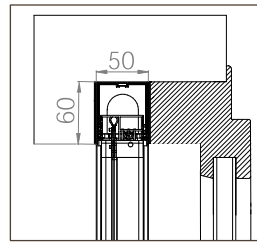
EINBAU-BORA TOP STANDARD 20/20
