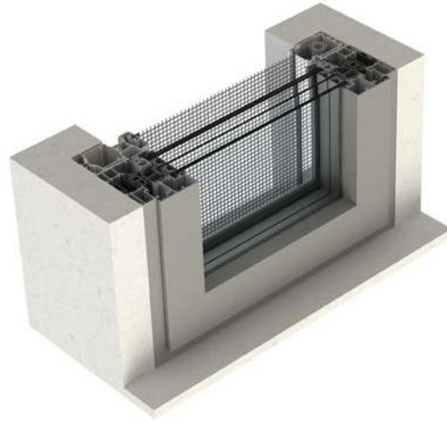
EINBAU-BORA TOP STANDARD 20/20
