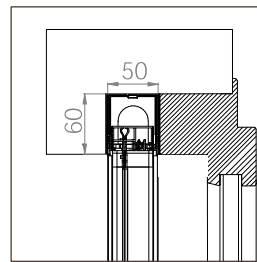
EINBAU-BORA STANDARD 50/50
