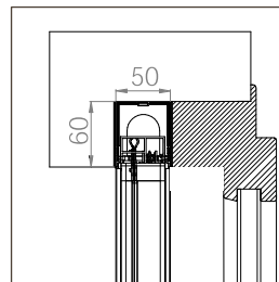
EINBAU-BORA SR STANDARD 50
